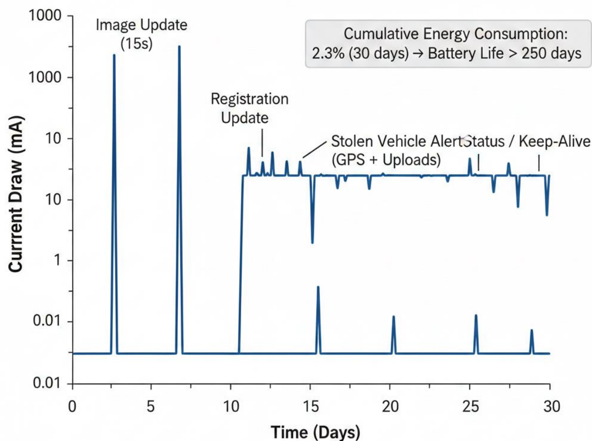
Figure 3: Power Consumption Over Time
