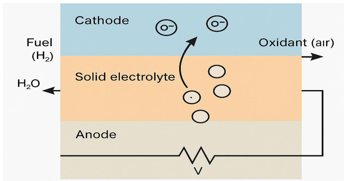
Fig. 3. Diagram of a solid-oxide fuel cell (SOFC).
